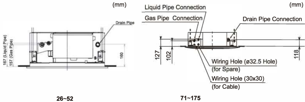
Fig. 3.6 Indoor Unit and Air Panel
