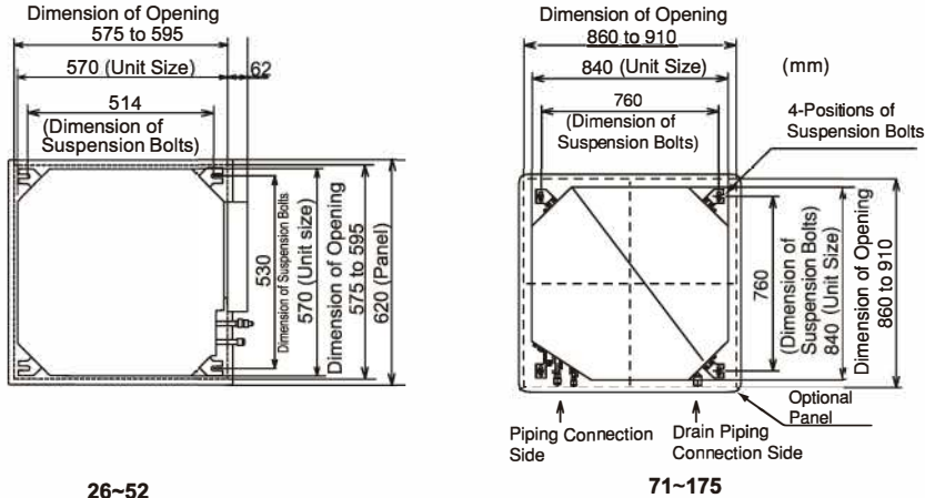
Fig. 3.3 Opening of False Ceiling and Suspension Bolts
