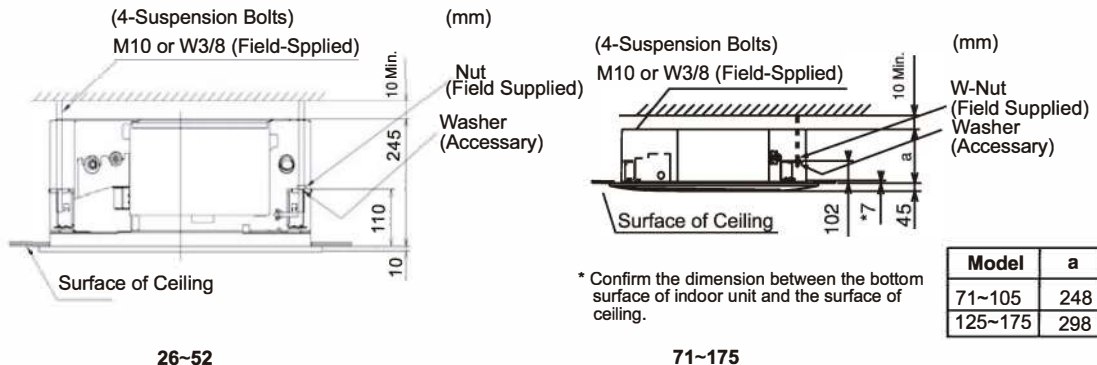
Fig. 3.5 Mounting Position
