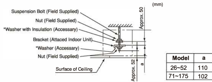
Fig. 3.7 Mounting Nuts and washer
