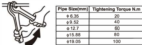
Fig. 4.2 Tightening Work of Flare Nut
