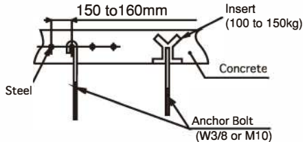
Fig. 3.4 Mounting Suspension Bolts
