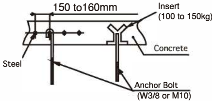
Fig. 3.4 Mounting Suspension Bolts
