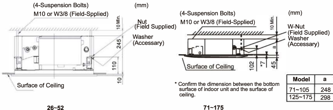
Fig. 3.5 Mounting Position
