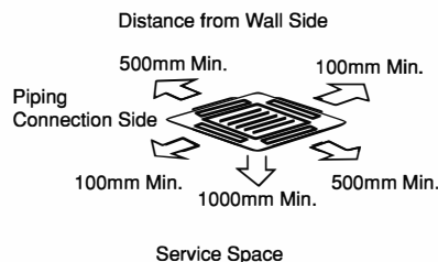
Fig. 3.1 Space around Indoor Unit
